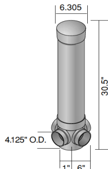
Diverter Valve
