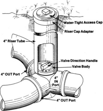
BullRun Valve
