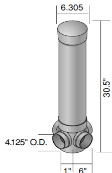
Diverter Valve
