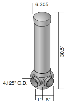
Diverter Valve
